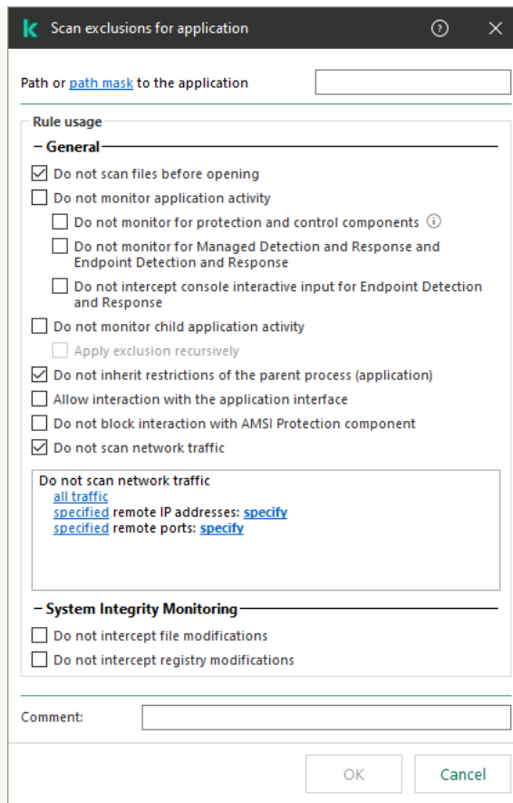
Trusted application settings
