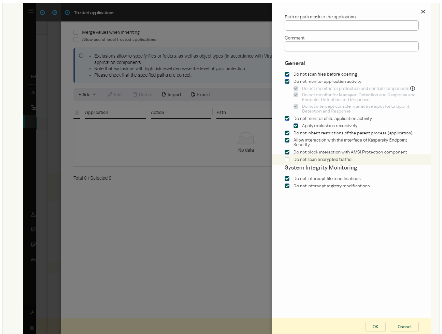
Trusted application settings
