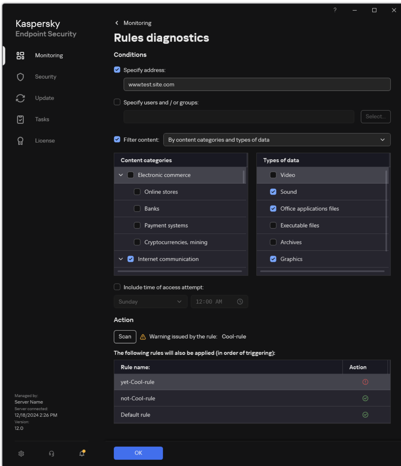
Web resource access test result
