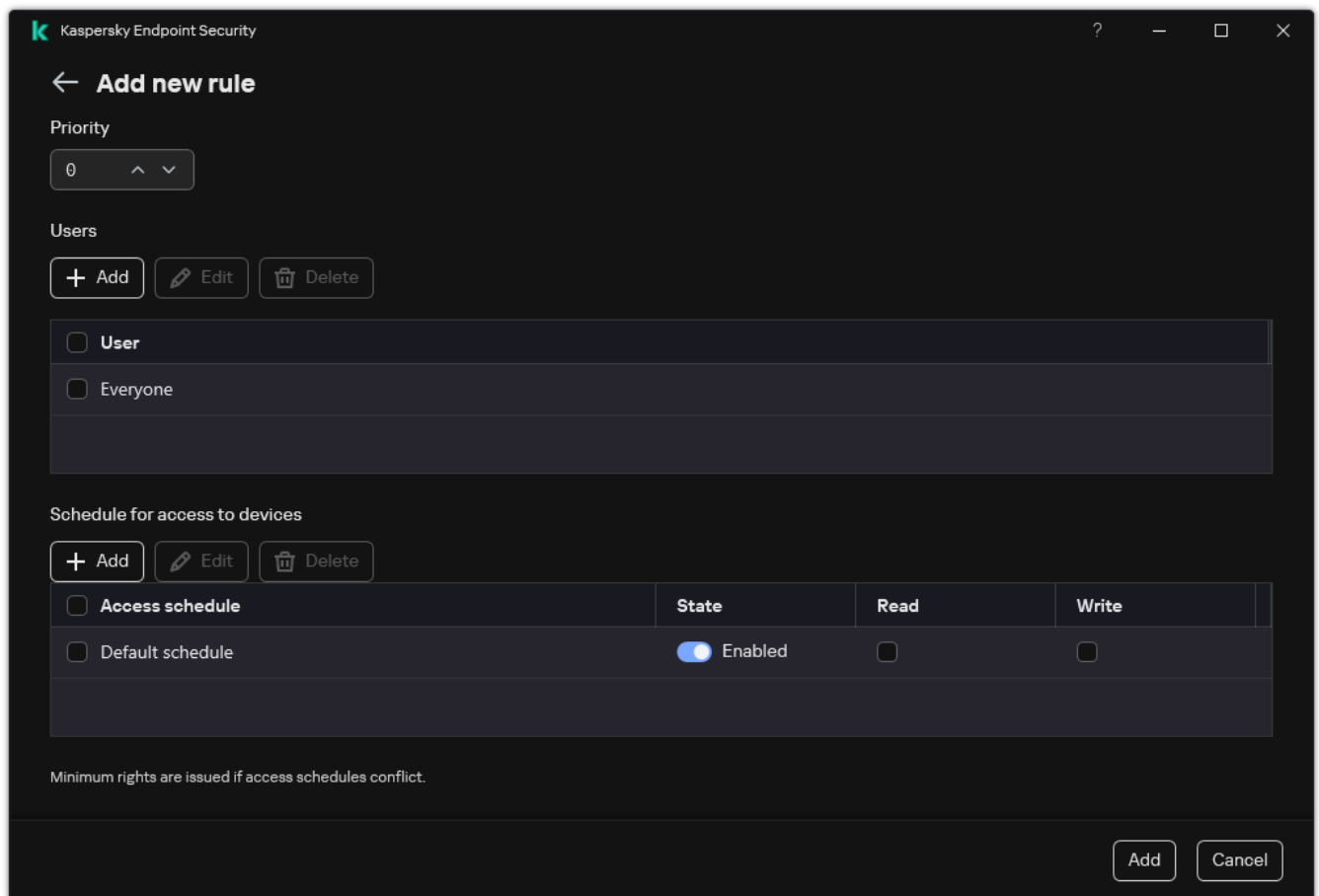
Device Control rule settings
