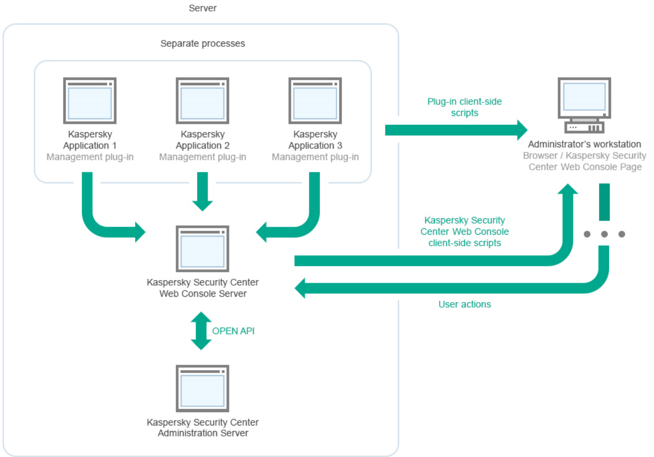
Deployment diagram of Kaspersky Security Center Administration Server and Kaspersky Security Center 13 Web Console
