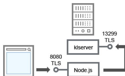
Administrationsserver und Kaspersky Security Center 14 Web Console
